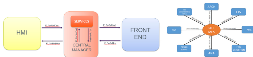
Figure 1 – Site MCS internal data flow and External interfaces
